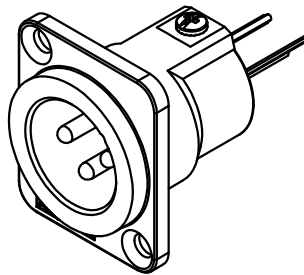
ISO VIEW
