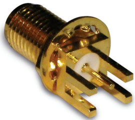
PCB SMA
